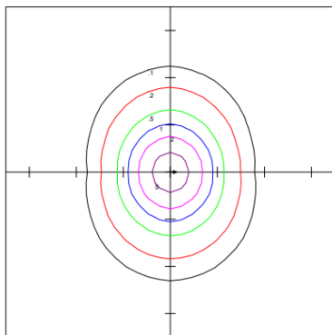
LNS-4FT-25-T1-F @10FT Set At 25W,5000K Distribution@10FT
