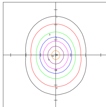
LNS-4FT-25-T1-F @10FT Set At 40W,5000K Distribution@10FT
