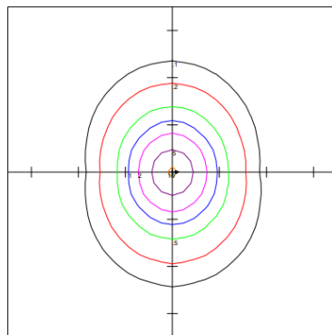
LNS-4FT-25-T1-F @10FT Set At 30W,5000K Distribution@10FT
